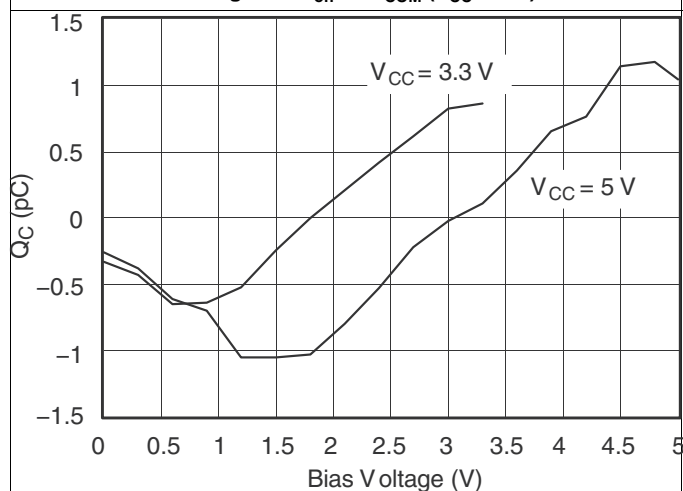
Figure 5. Charge Injection ( Q_C ) vs V_{COM}
