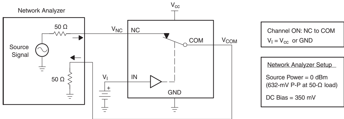
Figure 18. Bandwidth (BW)
