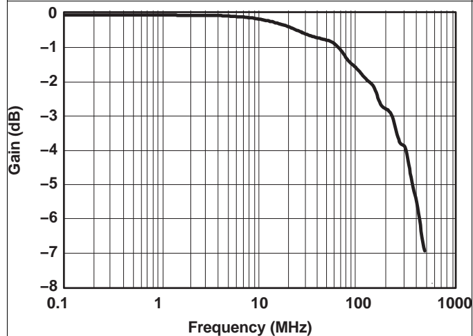
Figure 9. Gain vs Frequency ( V_{CC} = 5\text{ V} )
