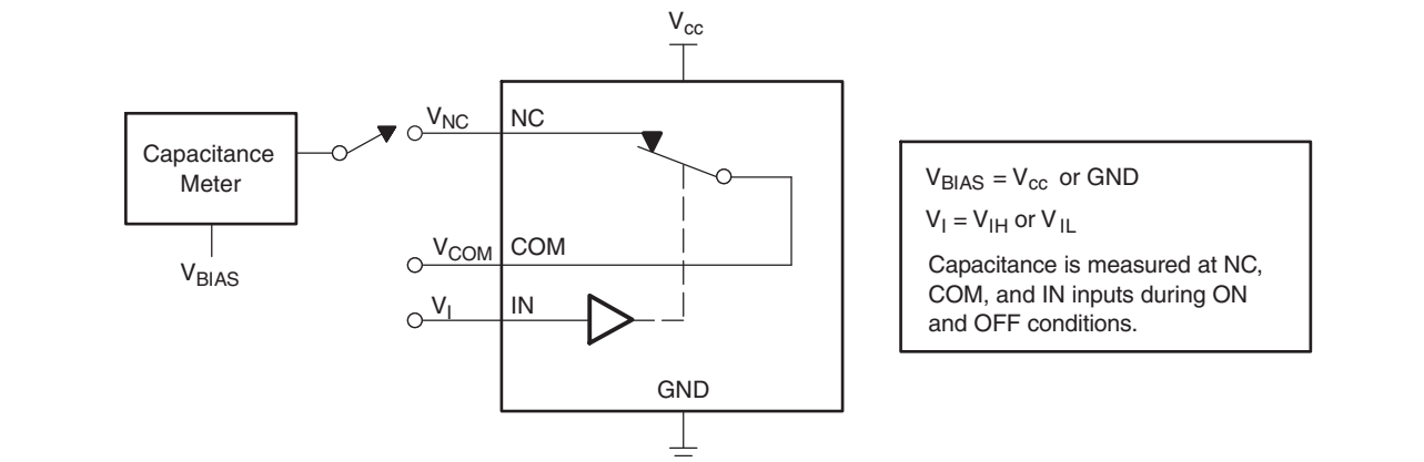
Figure 16. Capacitance ( C_I , C_{COM(OFF)} , C_{COM(ON)} , C_{NC(OFF)} , C_{NC(ON)} )
