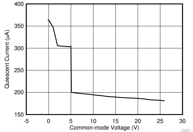
Figure 7-26. Quiescent Current vs. Common-Mode Voltage (INA180)
