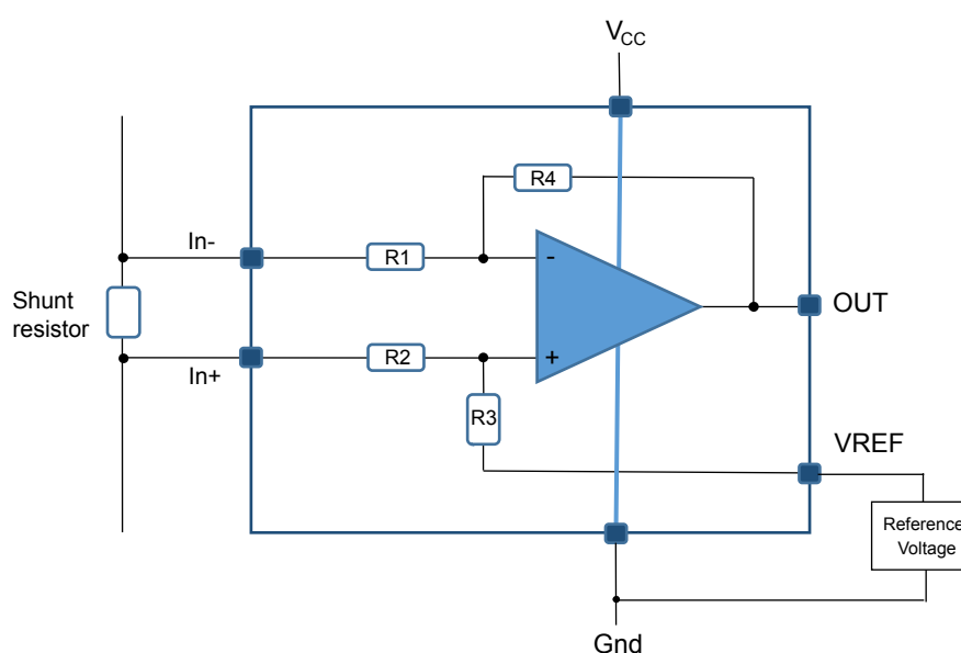
Figure 33. External supply
