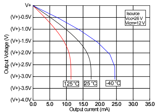
Figure 14. Positive output voltage swing vs. output current V_{CC} = 26\text{ V}
