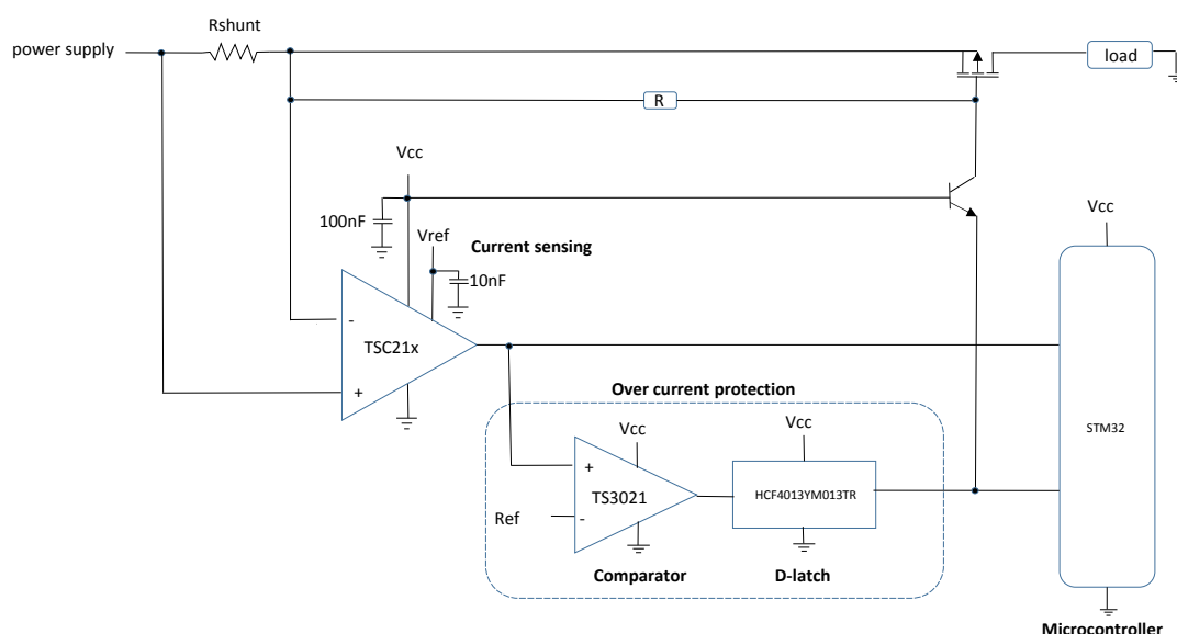
Figure 49. Power supply monitoring and OCP function
