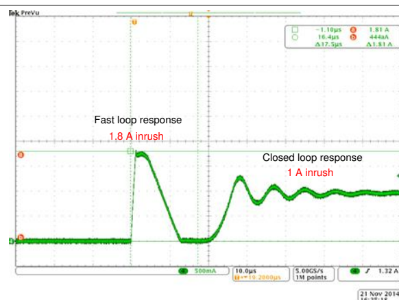
Figure 49. Hard Short-to-GND Waveform
