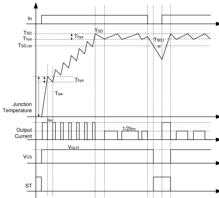
Figure 37. Thermal Behavior
