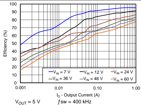
Figure 45. Light Load Efficiency
