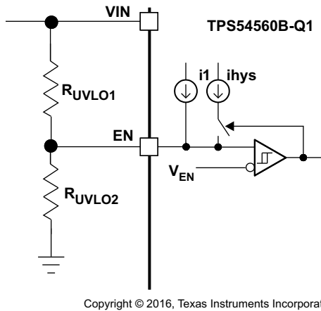
Figure 22. Adjustable Undervoltage Lockout (UVLO)
