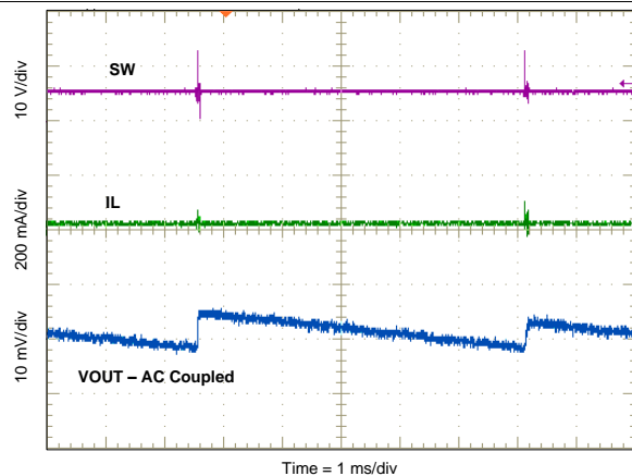
Figure 40. Output Ripple PSM
