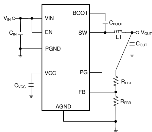
Simplified Schematic
