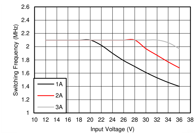
Figure 7-13. Switching Frequency versus Input Voltage V_{OUT} = 3.3\text{ V}
