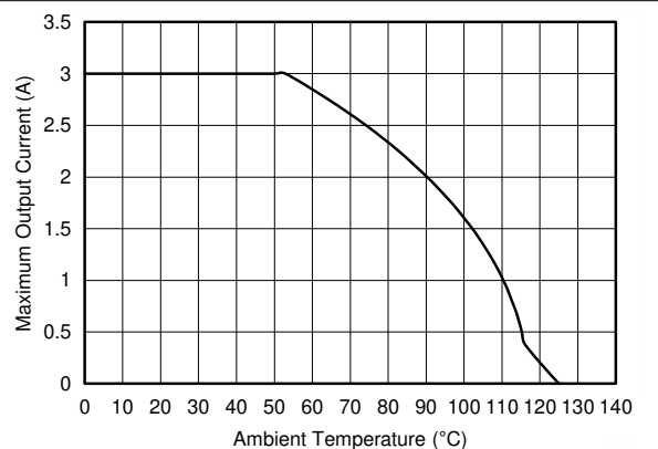
Figure 8-4. Maximum Output Current versus Ambient Temperature V_{IN} = 12\text{ V} V_{OUT} = 5\text{ V} f_{SW} = 400\text{ kHz} R_{\theta JA} = 50^\circ\text{C/W}
