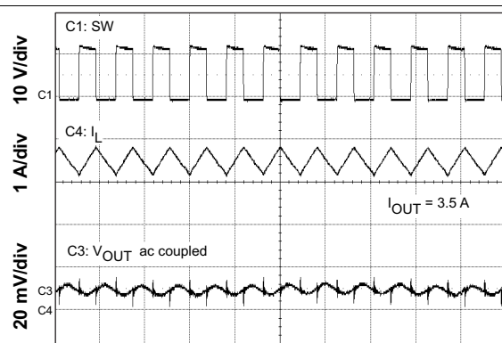
Time = 2 \mu s/div Figure 38. Output Ripple CCM
