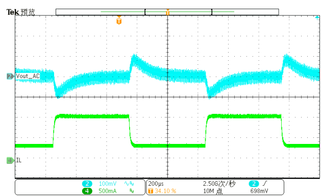
Figure 19. Load Transient (0.375A-1.125A, 1.6A/us)
