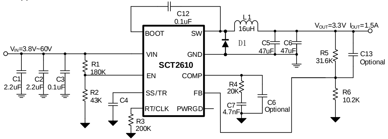
Figure 11. SCT2610Q Design Example, 3.3V Output with Programmable UVLO
