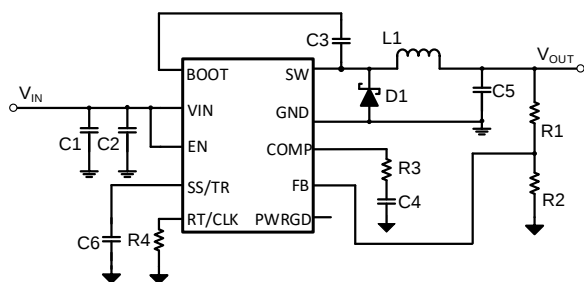
3.8V-60V, Asynchronous Buck Converter
