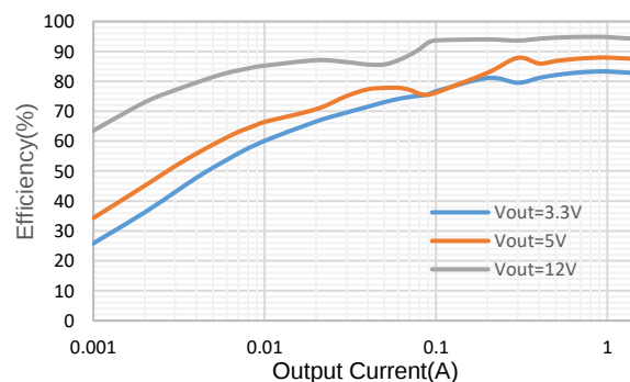
Efficiency, Vin=24V, Fsw=500KHz
