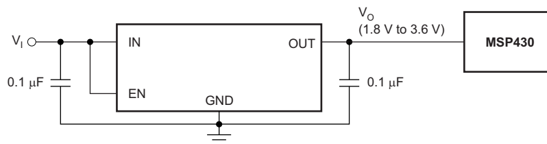
Figure 26. TLV713 Powering a Microcontroller
