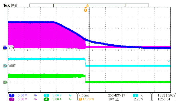
Figure 10. Power down
