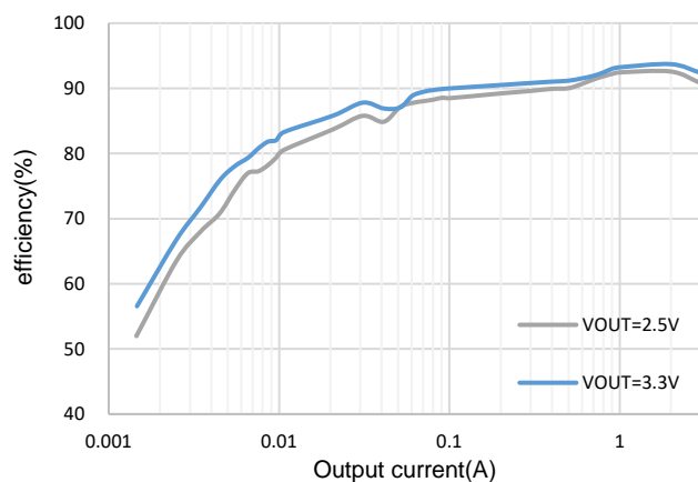
Figure 1. Efficiency vs Load Current(VIN=12V)
