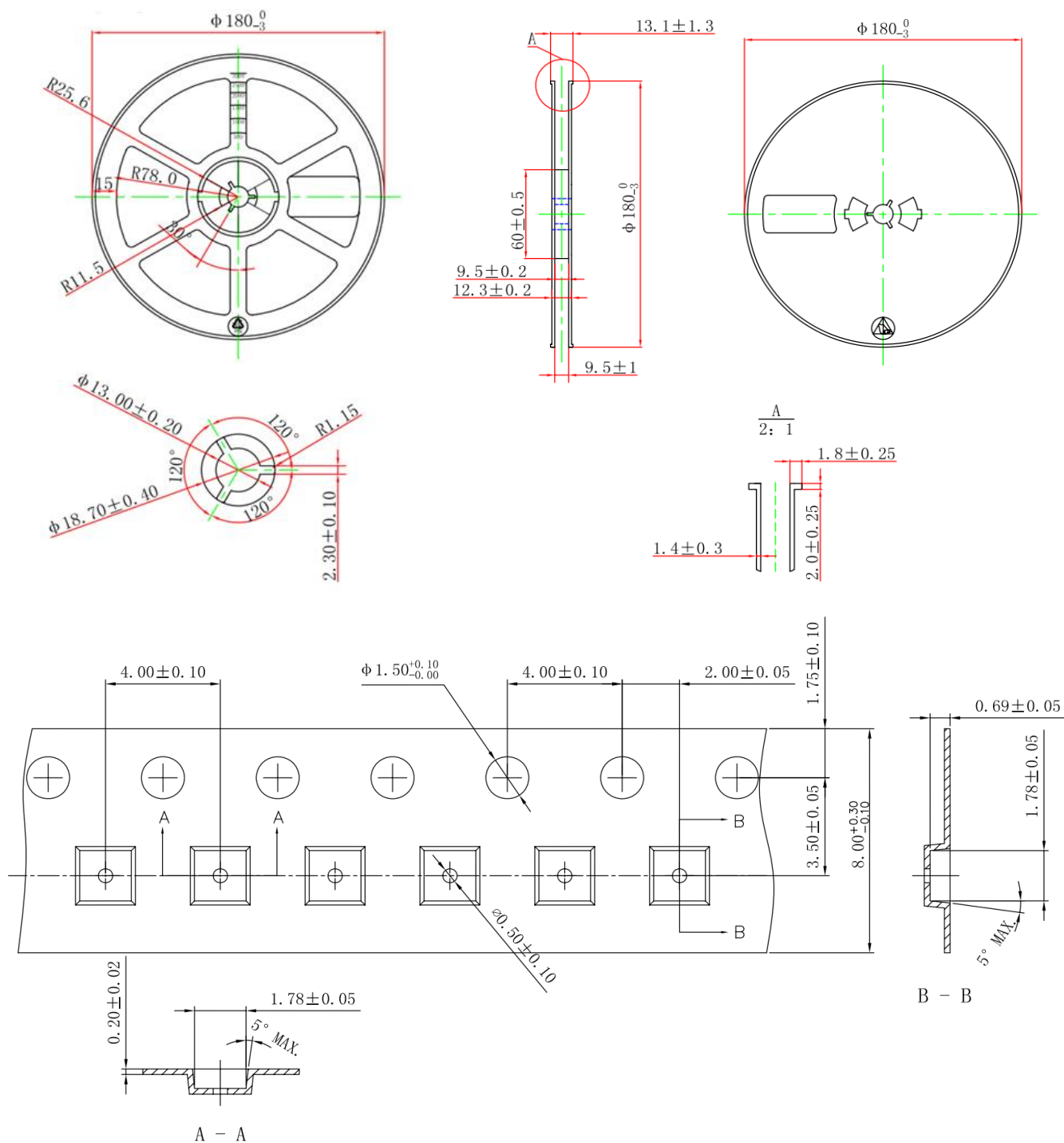
TAPE DIMENSIONS
