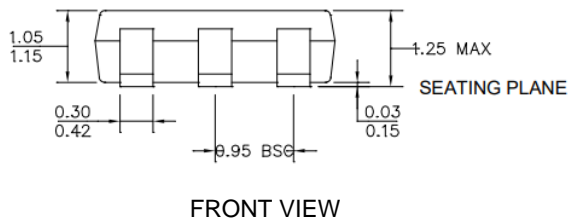
SOT23-6L Package Outline Dimensions
