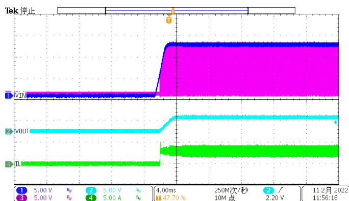
Figure 9. Power up
