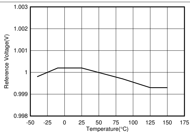
Figure 9. Reference Voltage versus Temperature
