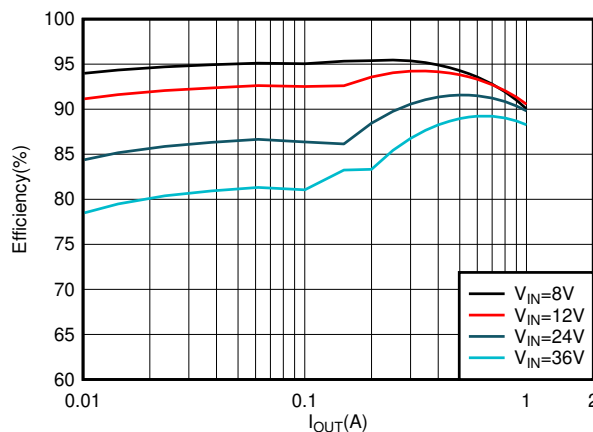
Efficiency versus Output Current V_{\text{OUT}} = 5 \text{ V} , 700kHz, PFM
