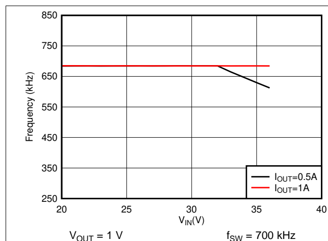
Figure 14. Frequency Foldback at T_{ON\_MIN}
