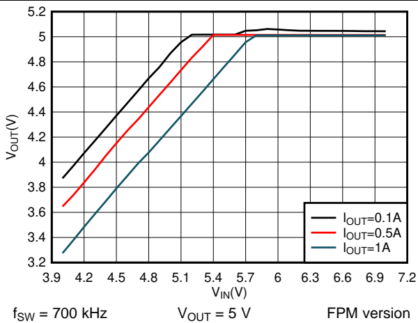
Figure 6. Dropout
