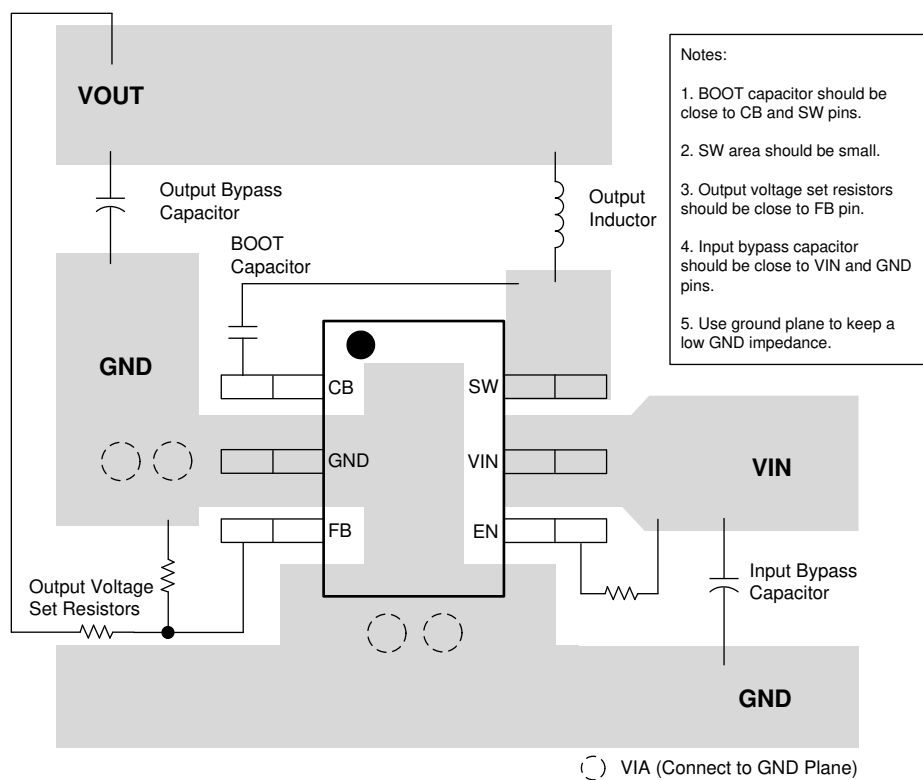
Figure 25. Layout
