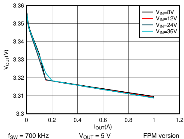
Figure 5. Line Regulation
