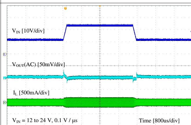
Figure 22. Line Transient
