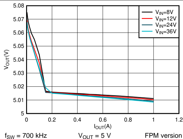
Figure 4. Load Regulation
