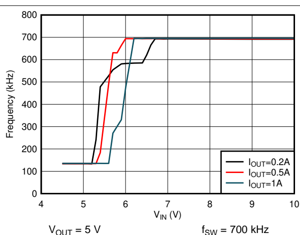
Figure 15. Frequency Foldback at T_{OFF\_MIN}
