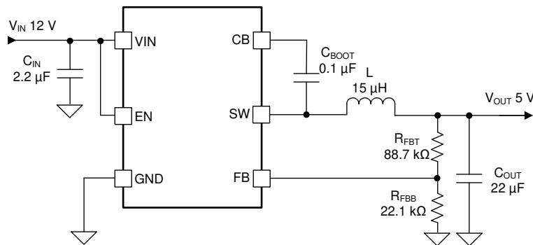
Figure 16. Application Circuit
