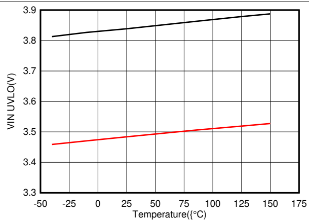
Figure 8. V_{IN} UVLO versus Temperature
