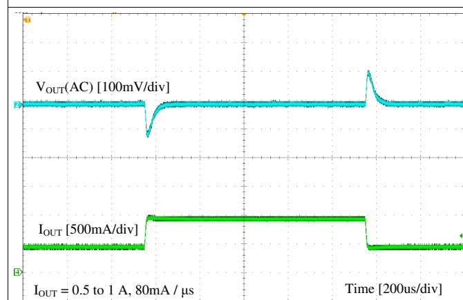
Figure 21. Load Transient
