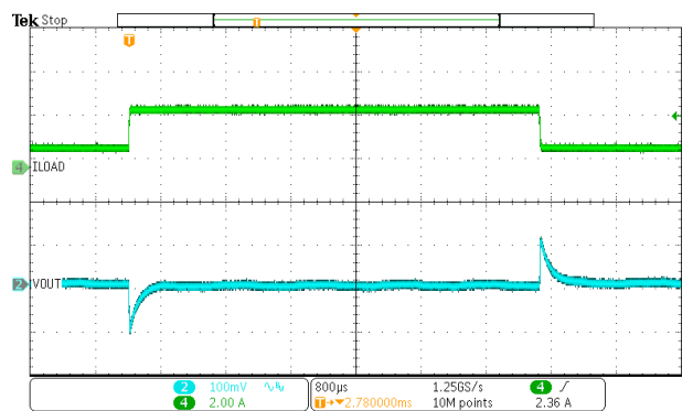
Figure 23. Load Transient (0.875A-2.625A, 250mA/us)
