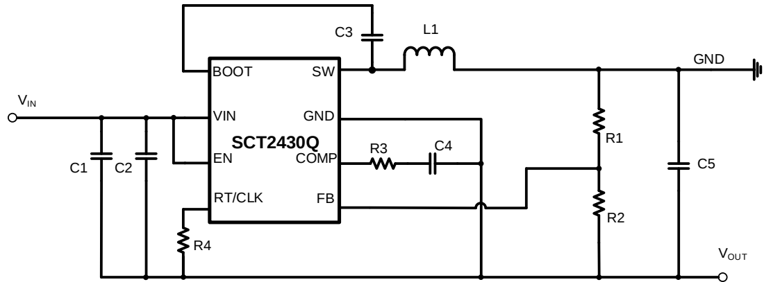
Figure 19. SCT2430Q Inverting Power Supply
