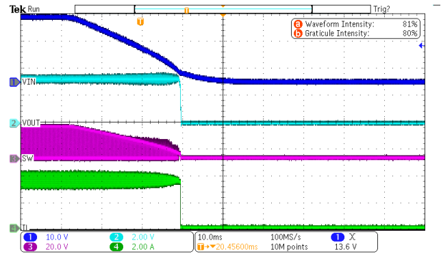
Figure 21. Power down
