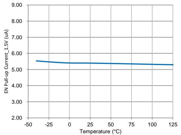
Figure 11. EN Pull-up Current vs Temperature
