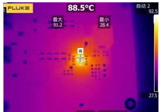
Figure 25. Thermal, 3.3Vout/3.5A
