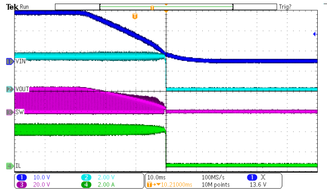
Figure 21. Power down
