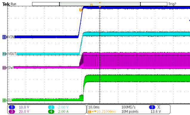
Figure 20. Power up
