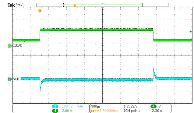
Figure 23. Load Transient (0.875A-2.625A, 250mA/us)
