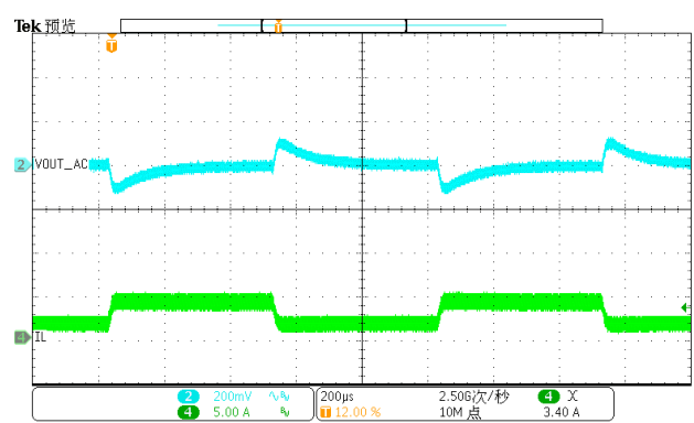
Figure 20. Load Transient (1.25A-3.75A, 1.6A/us)
