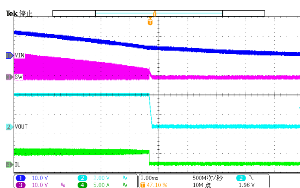
Figure 14. Power down(Iload=3.5A)
