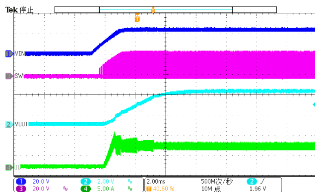
Figure 13. Power up(Iload=5A)
