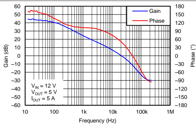
Figure 54. Overall Loop Frequency Response
