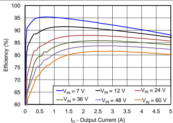
Figure 49. Efficiency vs Load Current
