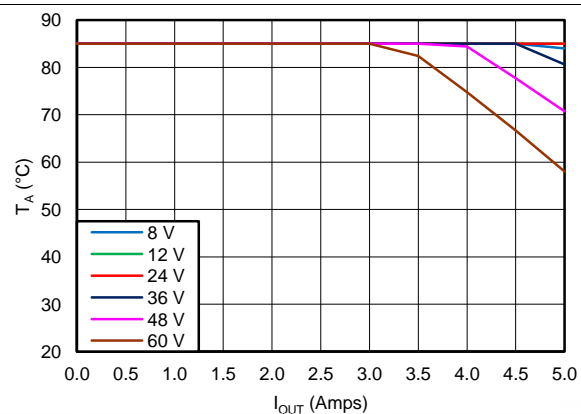
Figure 59. 5-V Outputs
