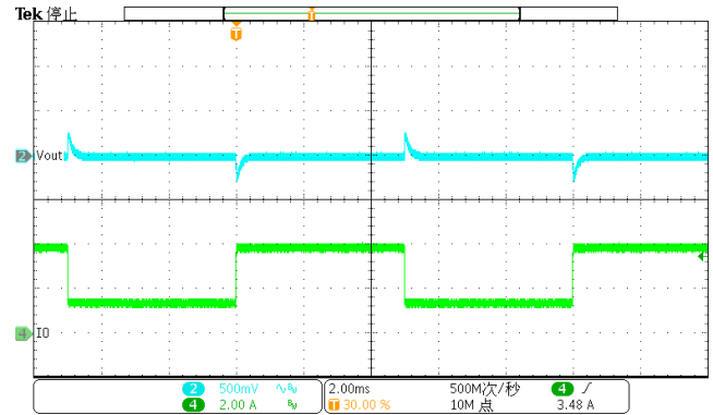
Figure 18. Load Transient (1.25A-3.75A, 1.6A/us)
