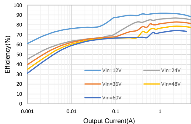
Efficiency, Vout=5V
