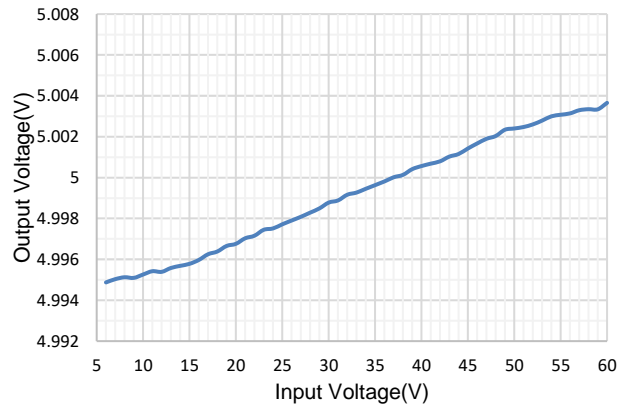
Figure 5. Line Regulation, Vout=5V, Iout=2.5A
