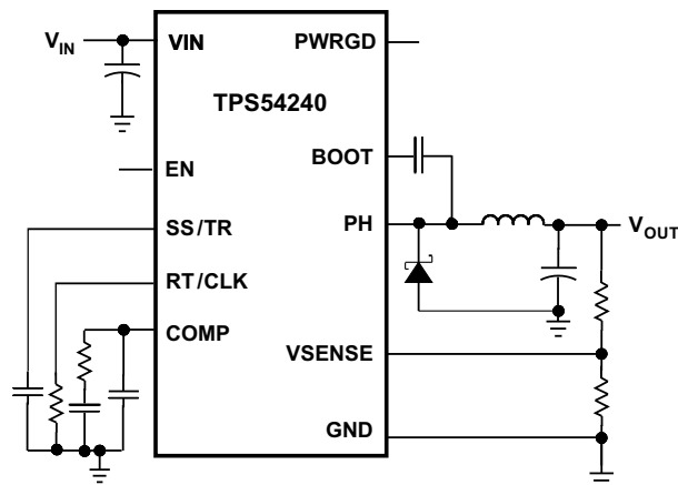
SIMPLIFIED SCHEMATIC
