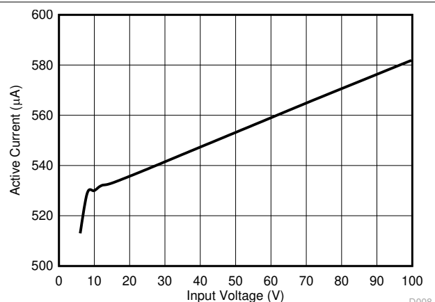
Figure 5-6. V_{\text{IN}} Active Current versus Input Voltage
