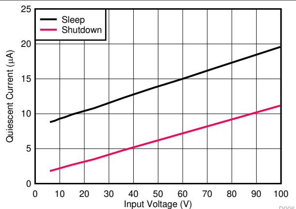
Figure 5-4. V_{\text{IN}} Shutdown and Sleep Supply Current versus Input Voltage
