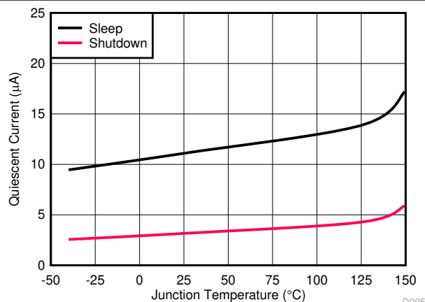
Figure 5-3. V_{\text{IN}} Shutdown and Sleep Supply Current versus Temperature
