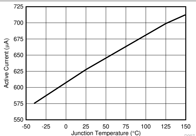
Figure 5-5. V_{\text{IN}} Active Current versus Temperature
