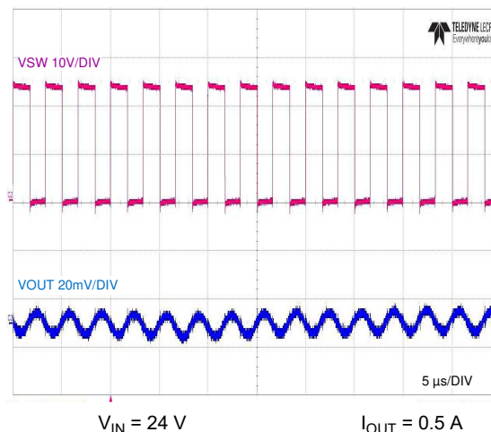
Figure 7-15. Full-Load Switching
