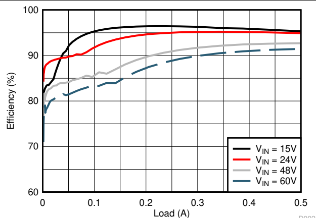
Figure 5-2. Conversion Efficiency (Linear Scale)
