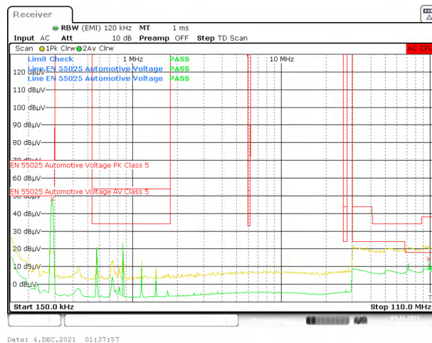
Figure 9-10. Full-Load Switching
