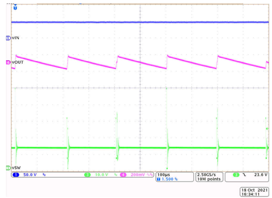
Figure 9-9. Light-load Switching
