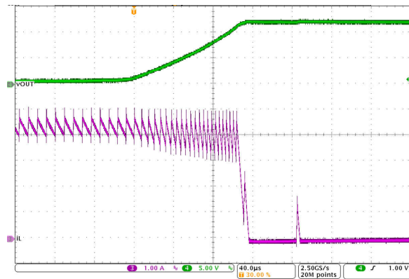
Figure 9-8. Short-Circuit Recovery
