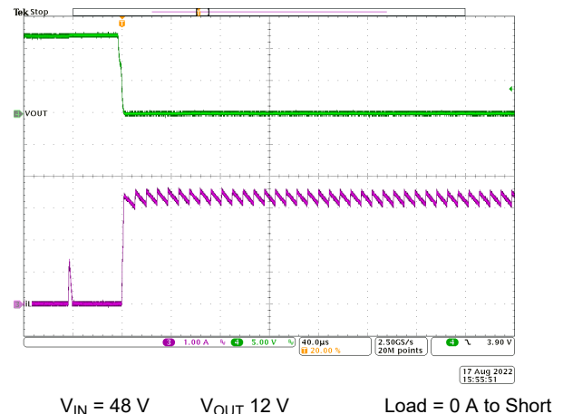
Figure 9-7. Short Circuit Applied
