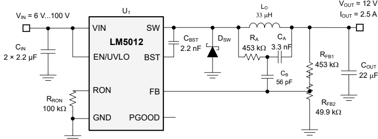
Typical Application
