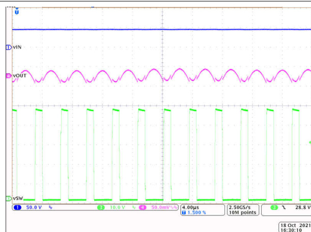
Figure 9-8. Short-Circuit Recovery
