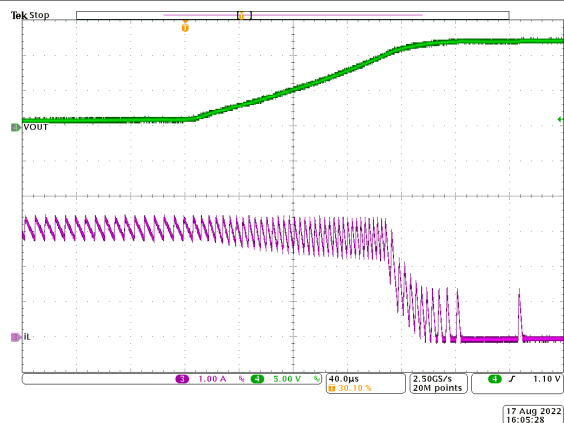
Figure 9-8. Short-Circuit Recovery
