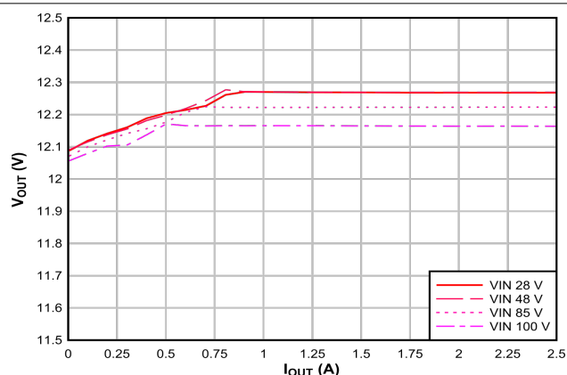
Figure 7-2. Load and Line Regulation
