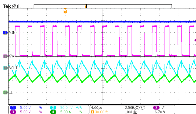
Figure 24. Steady-state (Iload=2A)
