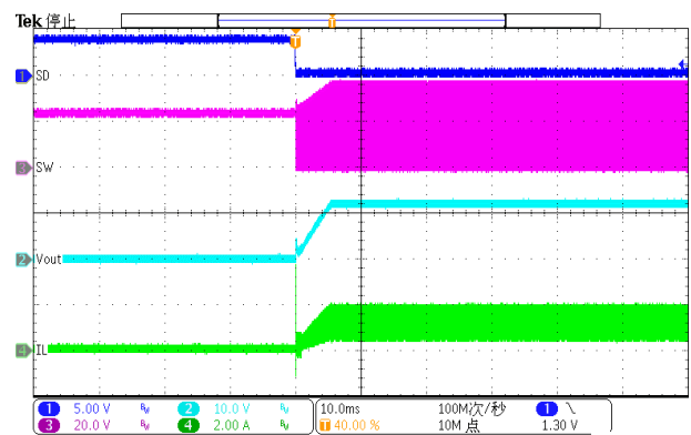
Figure 31. Shutdown remove
