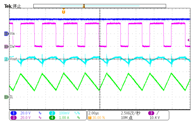
Figure 33. steady-state ( I_{load}=2A )
