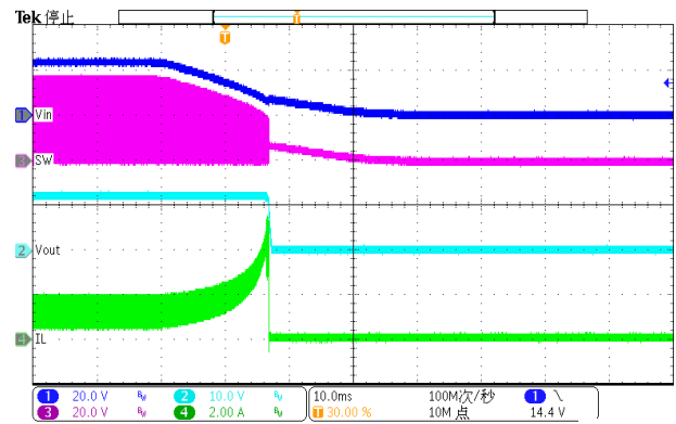
Figure 29. Power down( I_{load}=2A )
