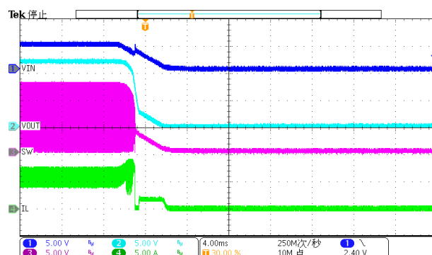
Figure 21. Power down(Iload=2A)
