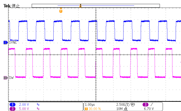
Figure 25. Sync Frequency
