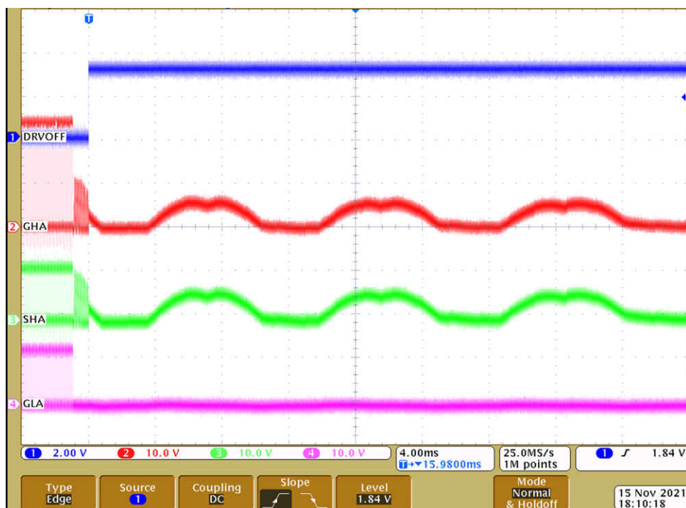
Figure 9-13. DRVOFF operation
