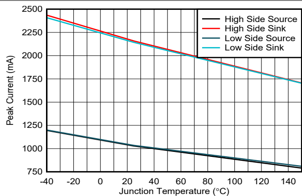
Figure 7-4. Driver Peak Current over Junction Temperature
