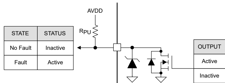
Figure 8-7. Open-Drain Output Pin Structure
