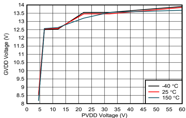
Figure 7-2. GVDD Voltage over PVDD Voltage
