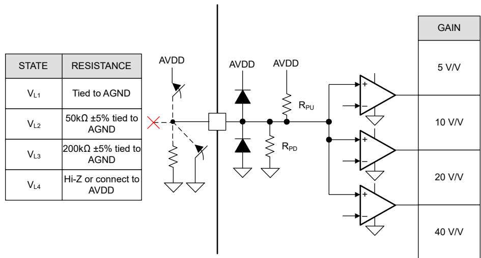
Figure 7-7. Four Level Input Pin Structure
