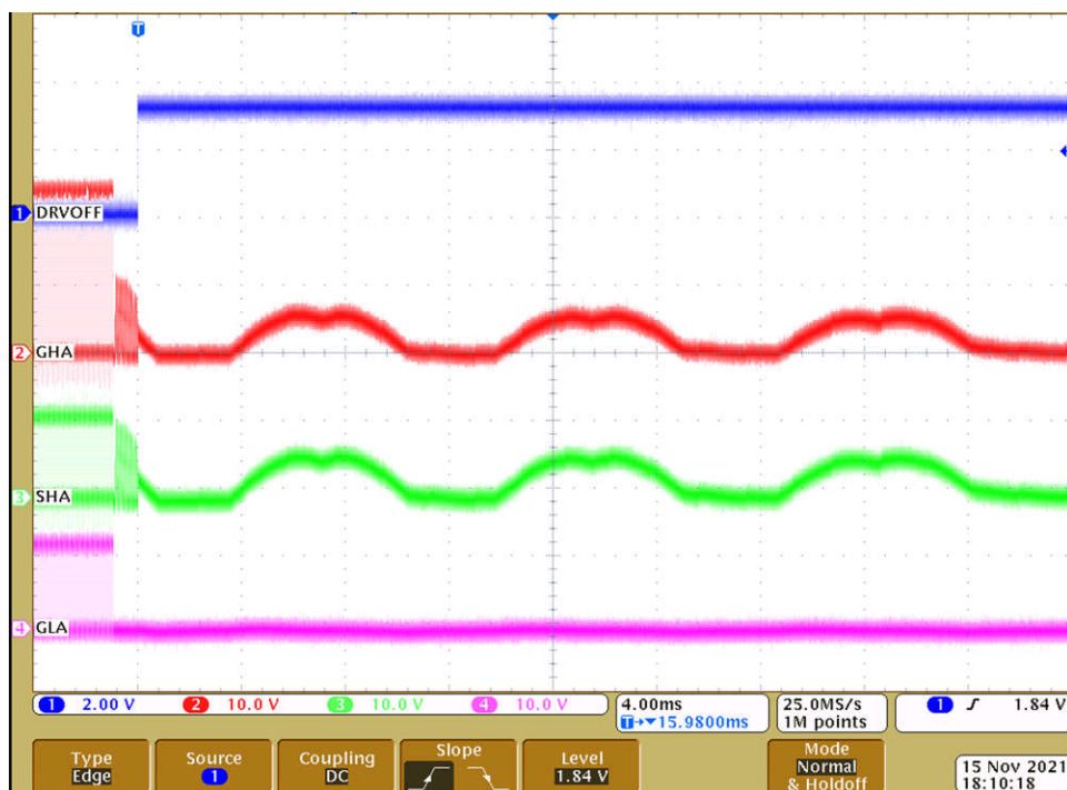
Figure 8-13. DRVOFF operation
