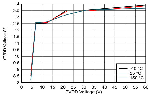
Figure 6-2. GVDD Voltage over PVDD Voltage
