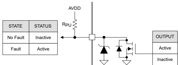
Figure 7-8. Open-Drain Output Pin Structure
