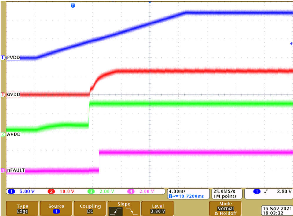
Figure 8-12. AVDD powerup
