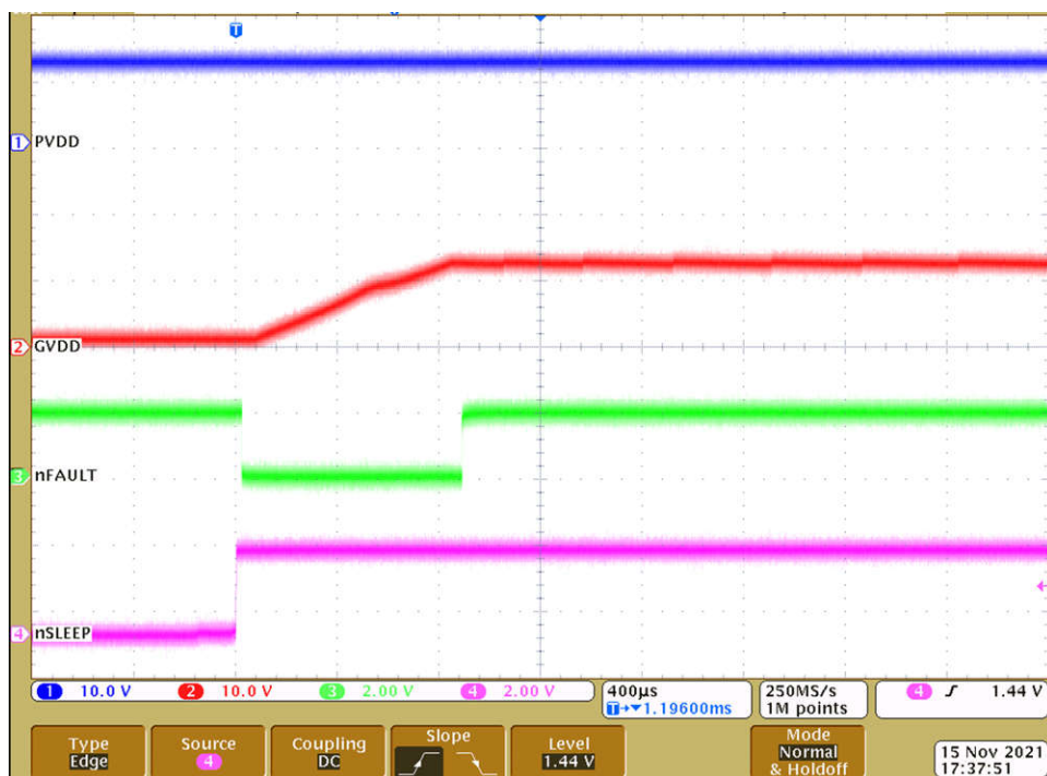
Figure 8-9. Device Powerup with nSLEEP
