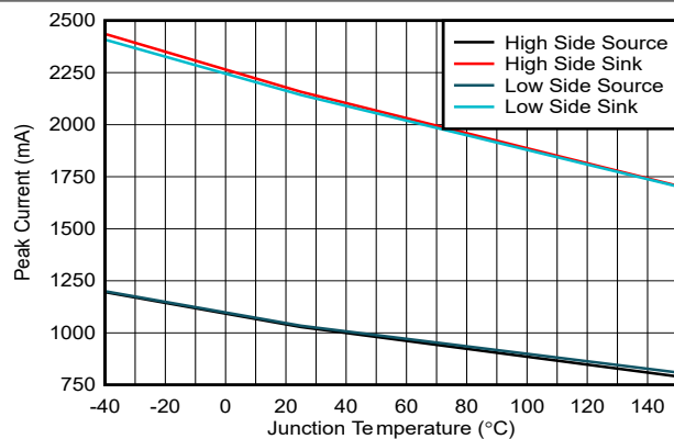
Figure 6-4. Driver Peak Current over Junction Temperature
