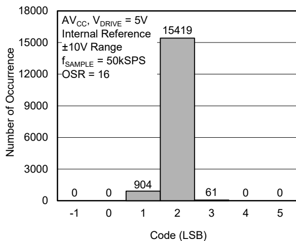
Figure 21. Histogram of Codes (OS × 16)
