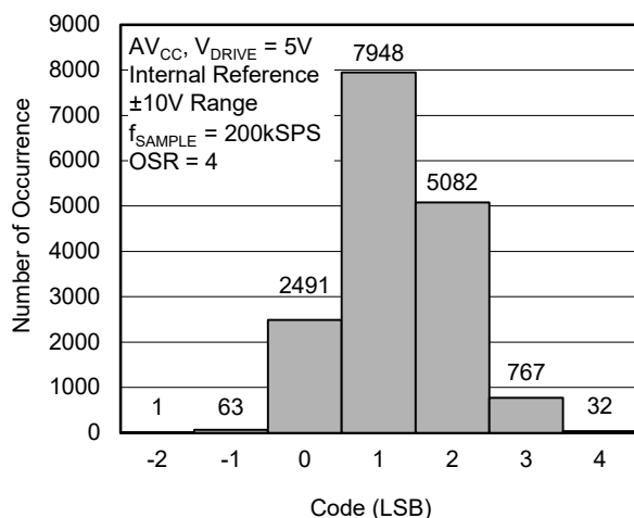
Figure 19. Histogram of Codes (OS × 4)
