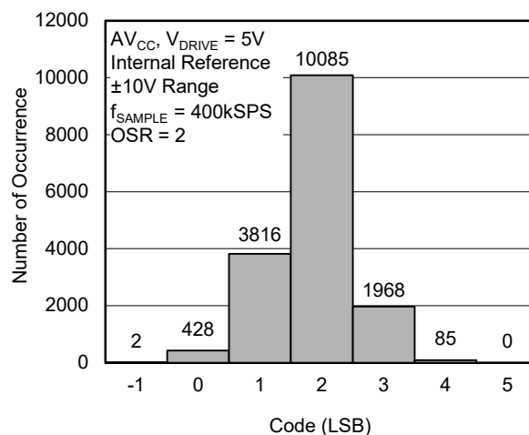
Figure 18. Histogram of Codes (OS × 2)
