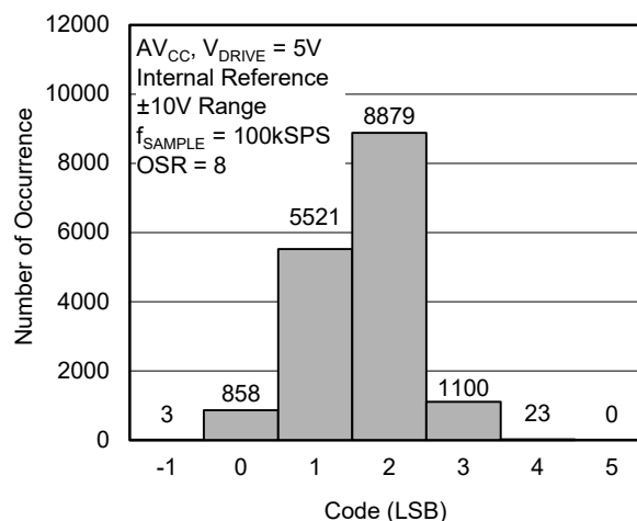
Figure 20. Histogram of Codes (OS × 8)
