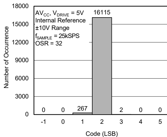
Figure 22. Histogram of Codes (OS × 32)
