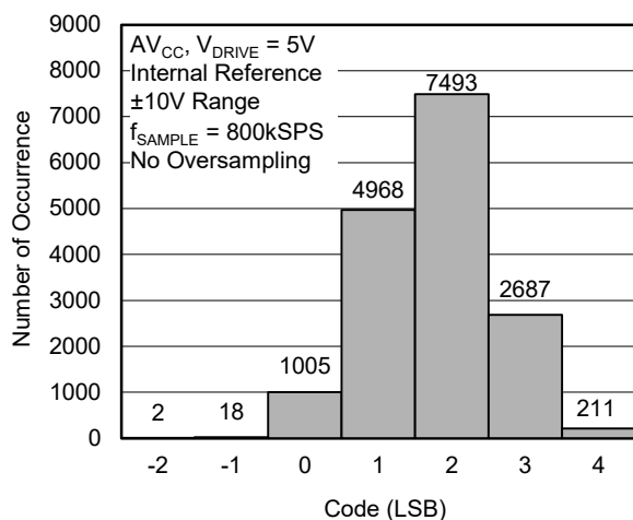
Figure 17. Histogram of Codes (No OS)
