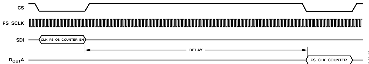
Figure 84. FS_CLK_COUNTER Functionality
