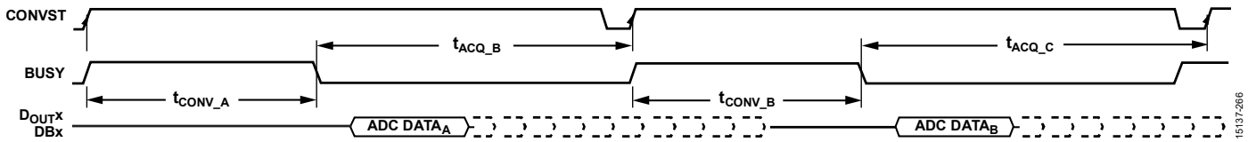
Figure 64. ADC Data Read After Conversion and/or During Conversion
