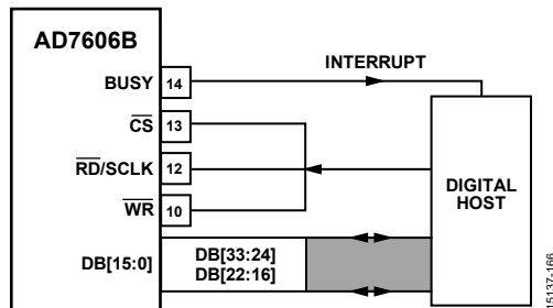
Figure 63. AD7606B Interface Diagram—One AD7606B Using the Parallel Bus, with \overline{CS} and \overline{RD} Shorted Together
