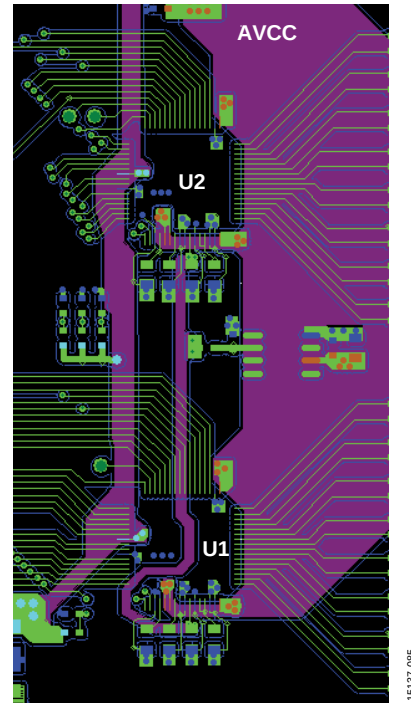
Figure 91. Layout for Multiple AD7606B Devices—Top Layer and Supply Plane Layer
