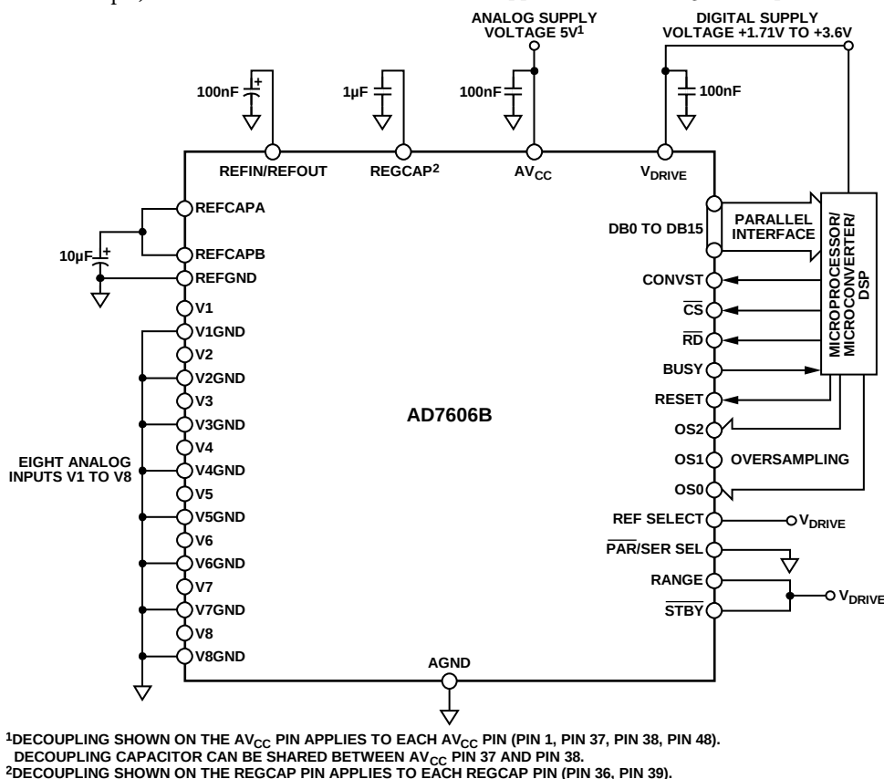
Figure 86. AD7606B Typical Connection Diagram, Hardware Mode
