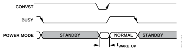
Figure 51. Autostandby Mode Operation
