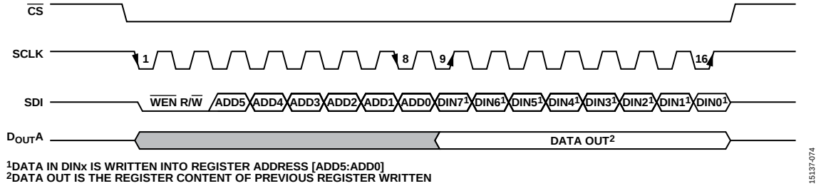
Figure 76. Serial Interface, Single-Write Command; SDI Clocks in the Address [ADD5:ADD0] and the Register Content [DINx] During the Same Frame, DOUTA Provides Register Content Requested on the Previous Frame
