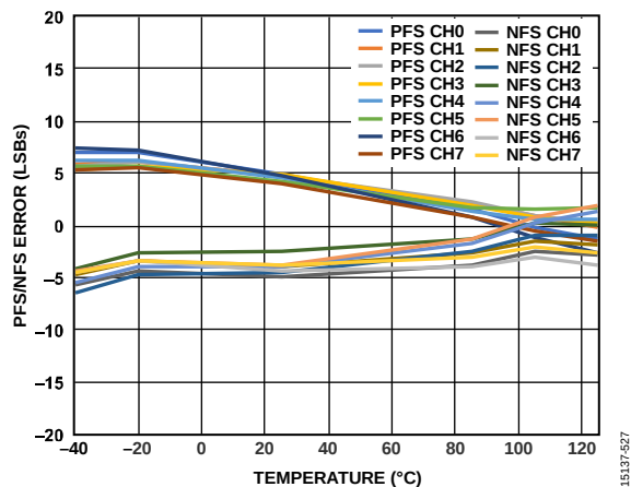
Figure 27. PFS/NFS Error vs. Temperature, \pm 10 V Range
