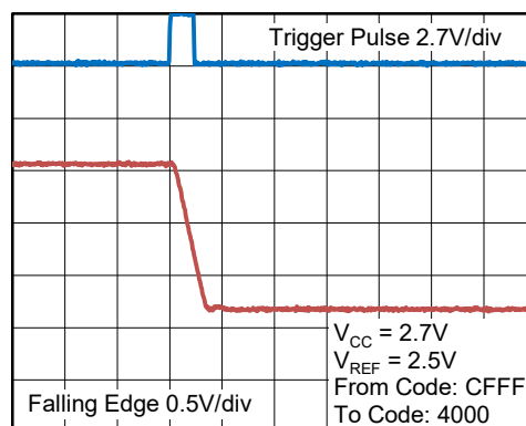
Half-Scale Settling Time: 2.7V Falling Edge
