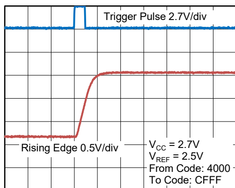
Half-Scale Settling Time: 2.7V Rising Edge
