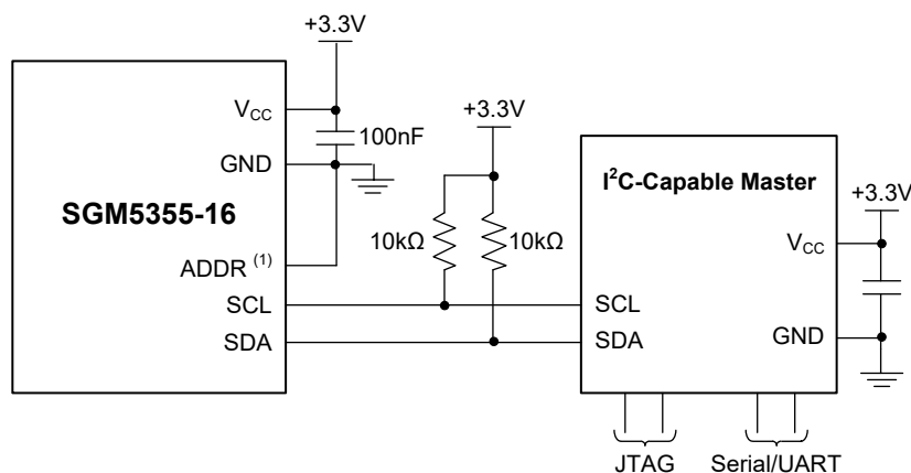
Figure 3. Basic Hardware Configuration
