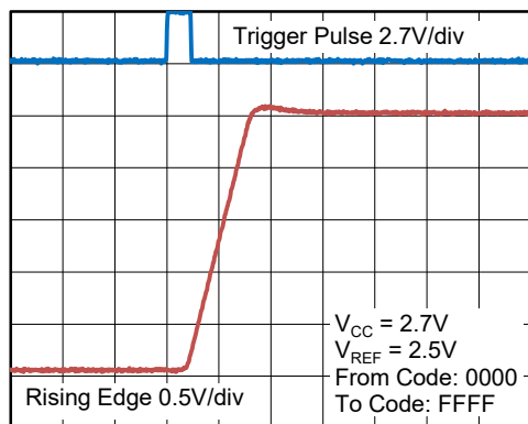
Full-Scale Settling Time: 2.7V Rising Edge
