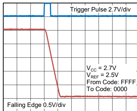
Full-Scale Settling Time: 2.7V Falling Edge
