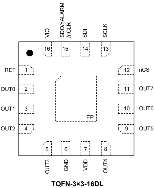
SGM71622R8/SGM71622R8A/SGM71622R8B (TOP VIEW)
