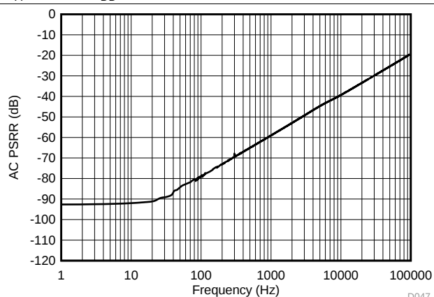
Figure 49. DAC Output AC PSRR vs Frequency
