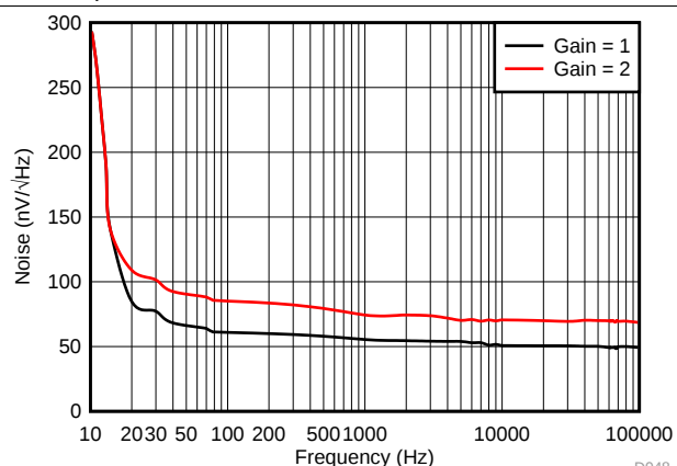
Figure 50. DAC Output Noise Density vs Frequency
