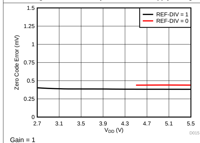
Figure 15. Zero Code Error vs Supply Voltage
