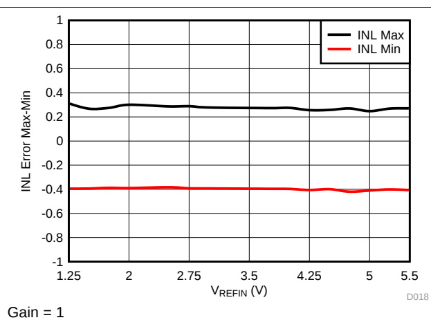
Figure 18. Integral Linearity Error vs Reference Voltage
