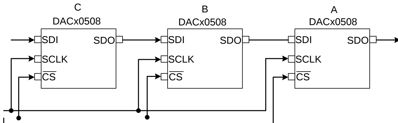
Figure 64. Daisy-Chain Layout
