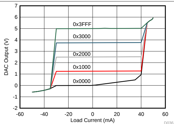
Figure 34. Source and Sink Capability with Gain = \frac{1}{2}
