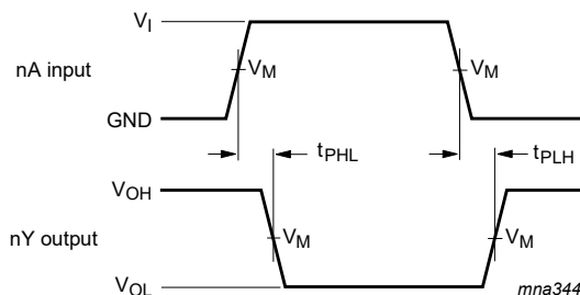
Fig. 4. The input (nA) to output (nY) propagation delay times
