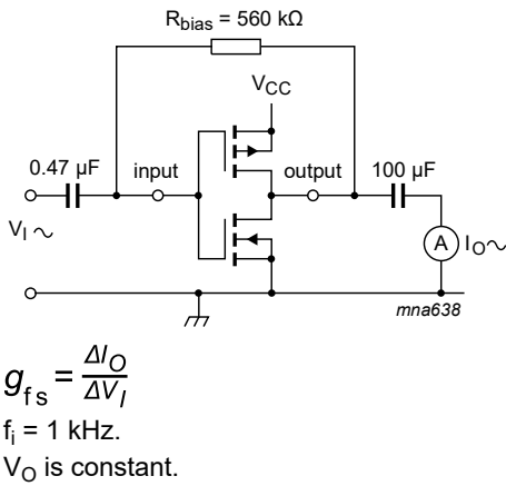
Fig. 7. Test set-up for measuring forward transconductance
