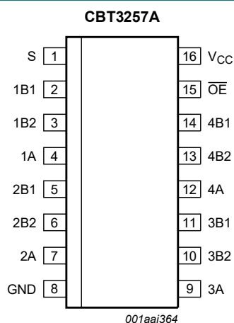
Fig. 2. Pin configuration SOT109-1 (SO16) and SOT519-1 (SSOP16)
