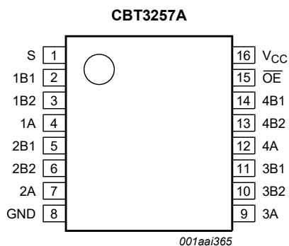
Fig. 3. Pin configuration SOT403-1 (TSSOP16)
