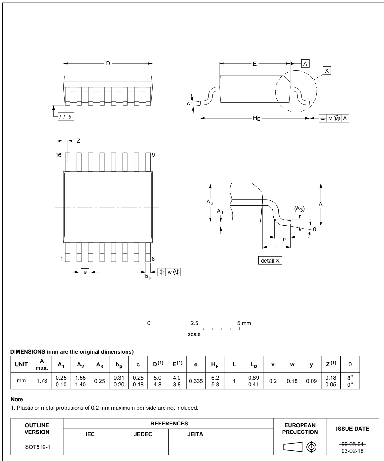
Fig. 9. Package outline SOT519-1 (SSOP16)
