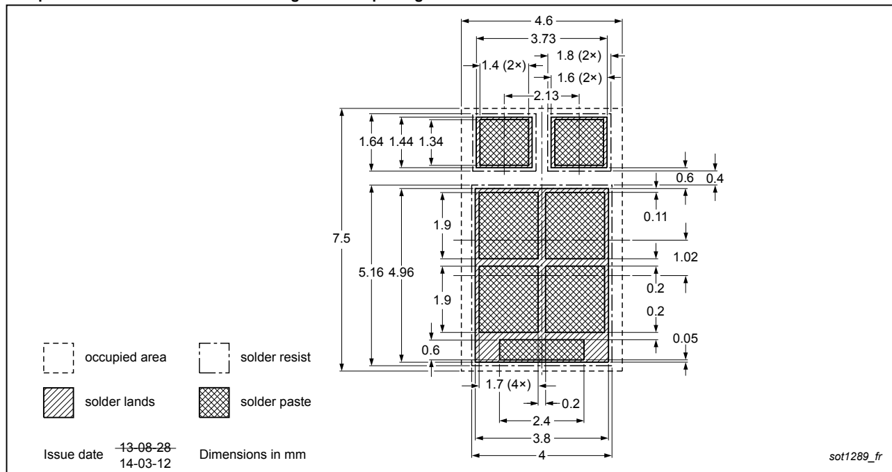
Fig. 18. Reflow soldering footprint for CFP15 (SOT1289)
