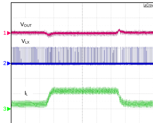
Load Transient
