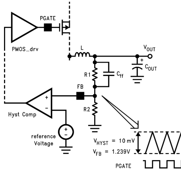
Figure 19. Hysteretic Window
