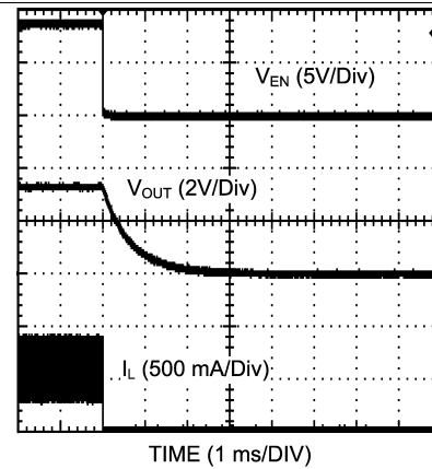
Figure 18. Shutdown Transient
