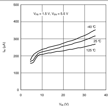
Figure 1. Quiescent Current vs Input Voltage
