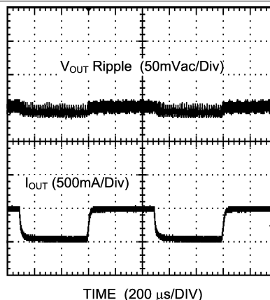
Figure 29. Load Transient
