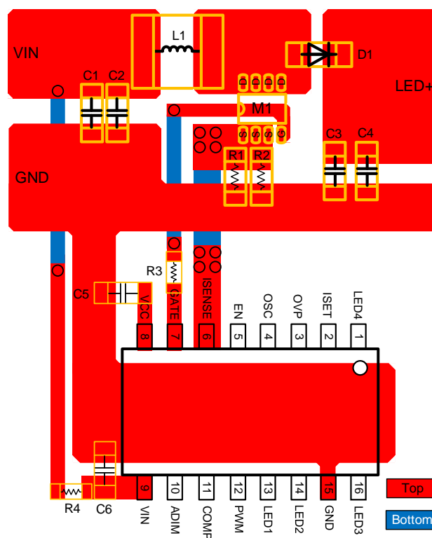
Figure 2: Recommended PCB Layout
