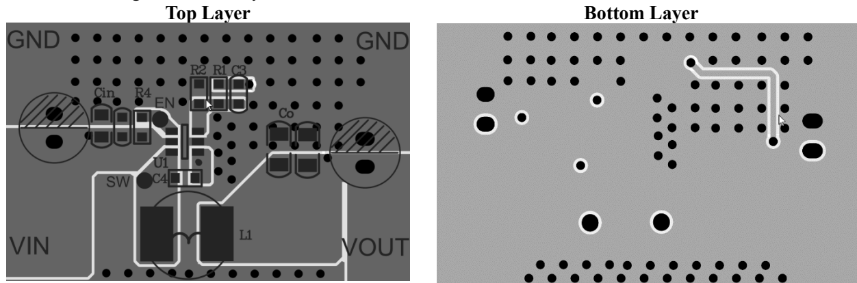
Figure 4. Sample of PCB Layout (EUP3152)
