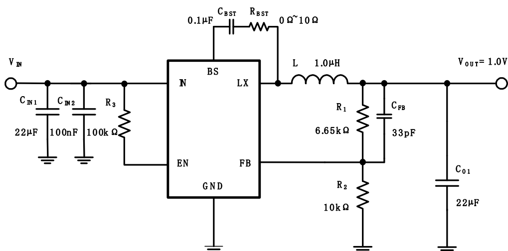
Figure 10. Application Circuits of 12V Input, 1V Output
