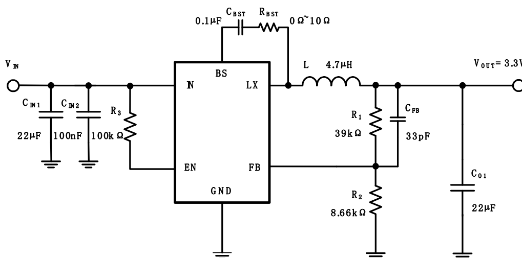
Figure 1. EUP3152 Typical Application Circuits
