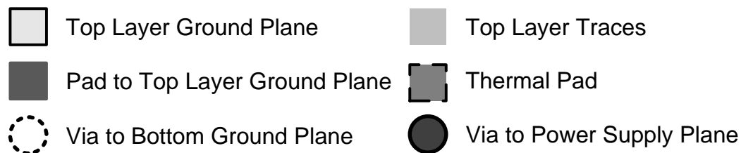
Figure 41. TPA2012D2 WQFN Layout Example
