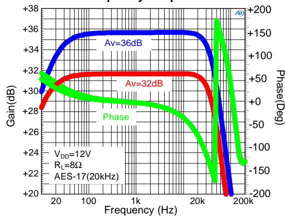
Frequency Response
