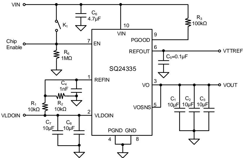
Figure 1. Schematic Diagram
