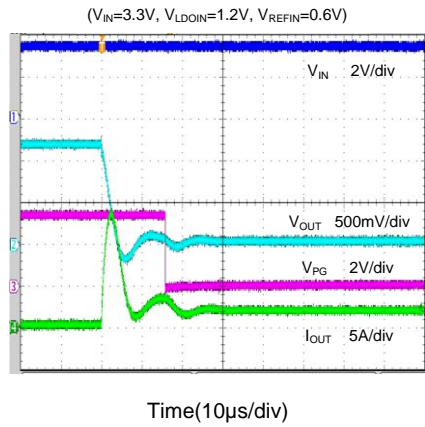
Short Circuit Response
